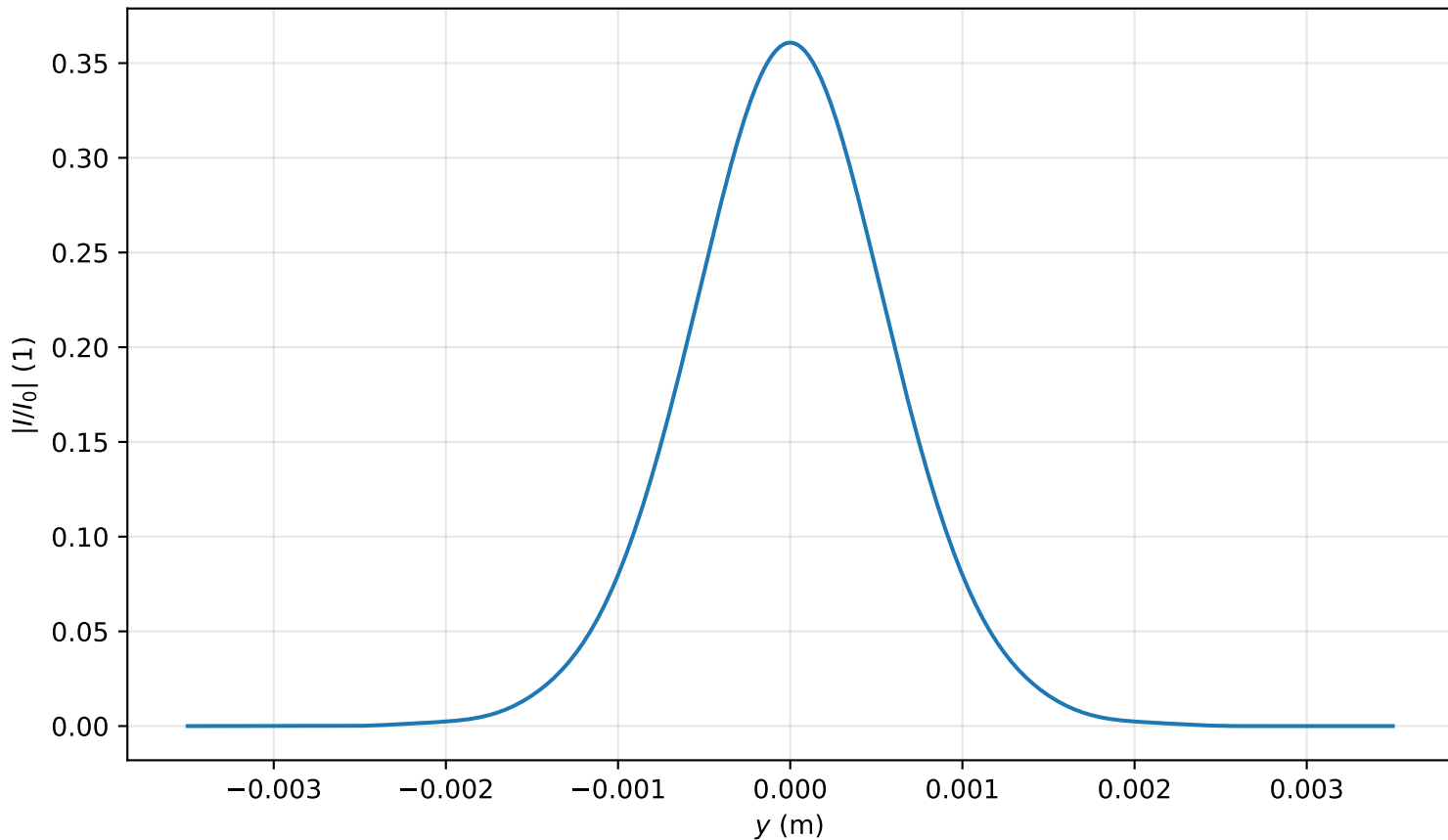
Intensity profile I(x=0, y, z=3.742)/I_0 , P_{in}=0.4P_{cr} , artificial time
